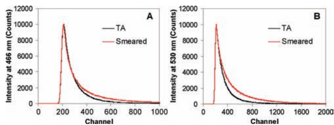
Figure 5. Fluorescence lifetime decays of a \text{BF}_2\text{dbmOC}_{12}\text{H}_{25} (control) solid film on a piece of weighing paper monitored at 466 nm (A) and 530 nm (B) ( \lambda_{\text{ex}} = 369 nm LED). TA: thermally annealed.
